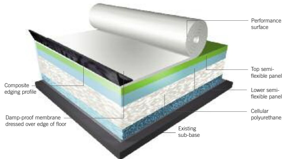
Cellular polyurethane layer First layer of semi-flexible panels Top semi-flexible panel layer with joints staggered Harlequin vinyl performance surface
